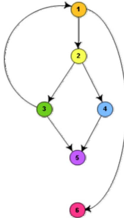
(b) Control Flow Graph
