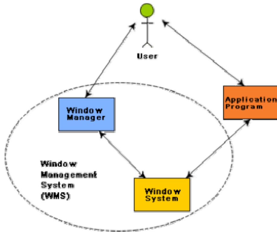
Fig. 9.7: Window Management System
