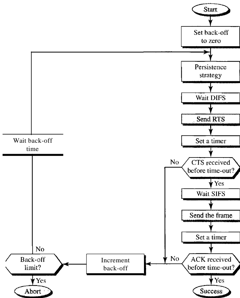
Figure 14.4 CSMA/CA flowchart
