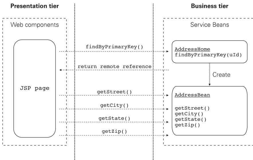
Figure 18.4 Accessing attributes remotely
