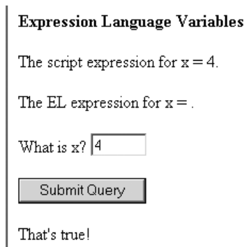
Figure 13.1 HTML output from EL_Variables.jsp
