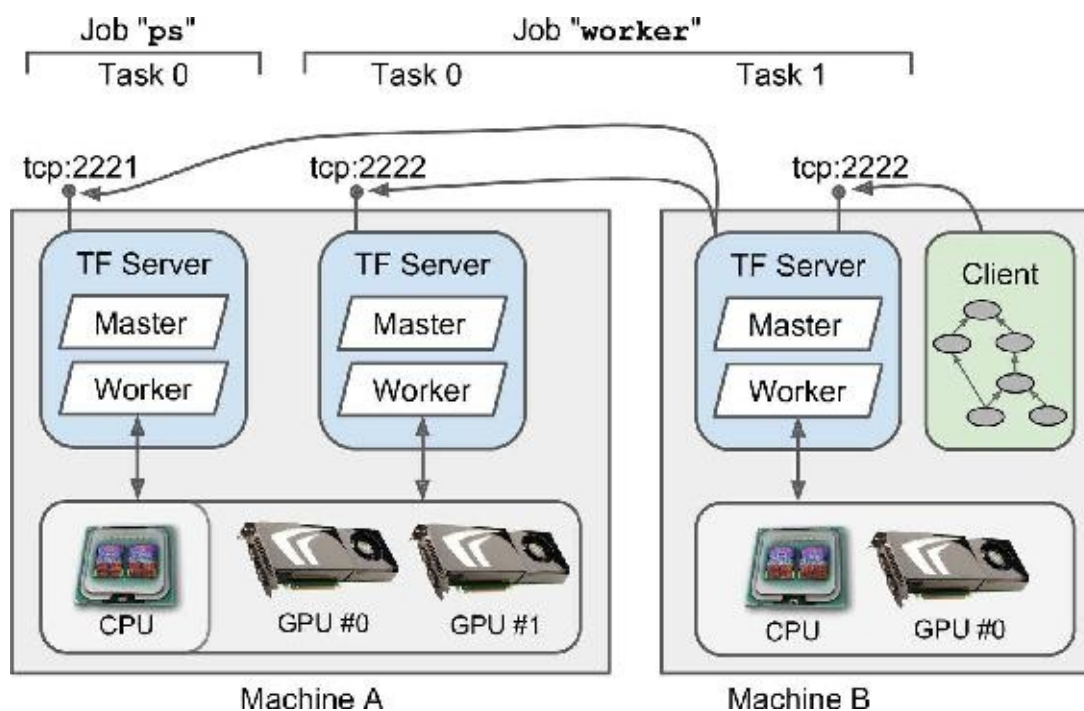
Figure 12-6. TensorFlow cluster
