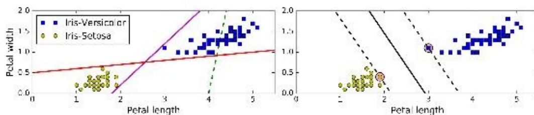
Figure 5-1. Large margin classification
