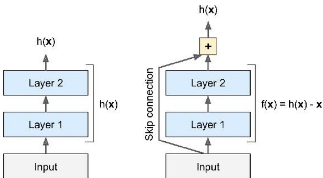
Figure 13-12. Residual learning
