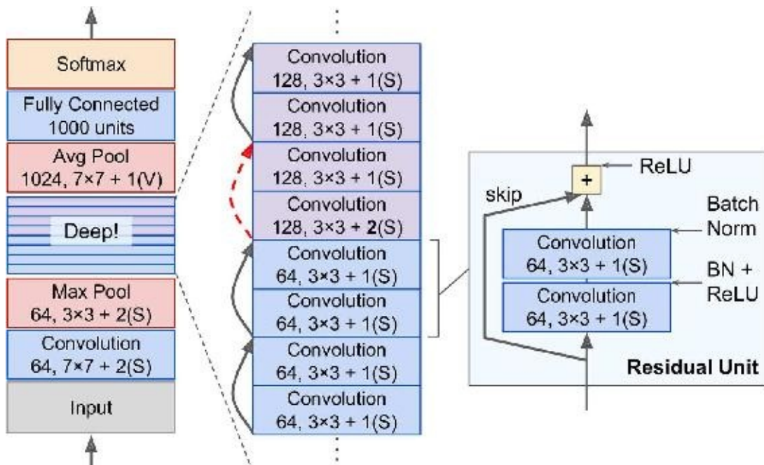
Figure 13-14. ResNet architecture
