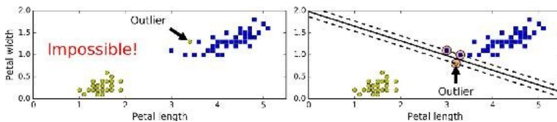
Figure 5-3. Hard margin sensitivity to outliers
