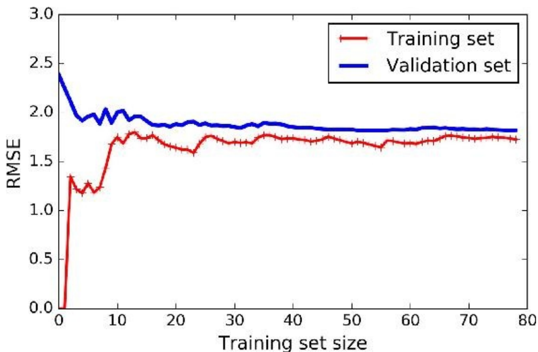
Figure 4-15. Learning curves
