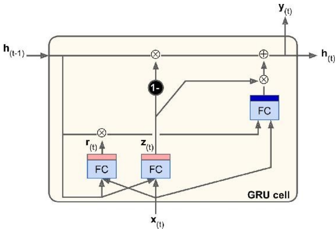
Figure 14-14. GRU cell
