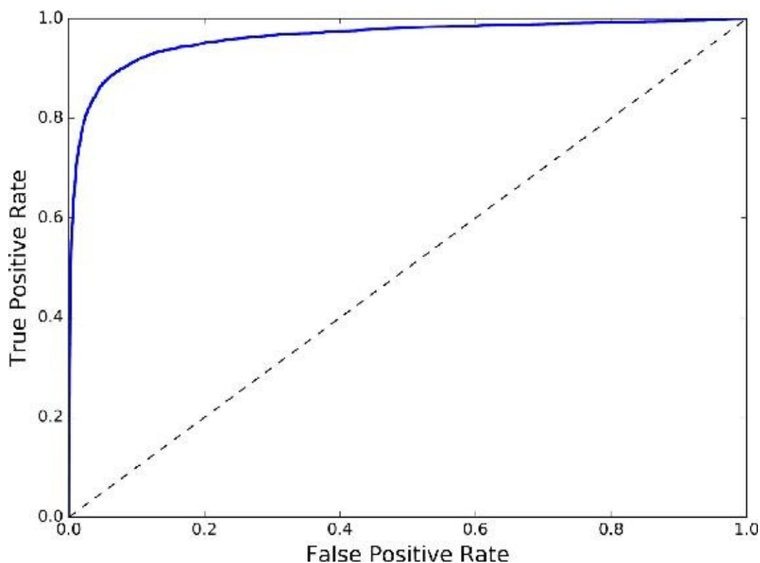
Figure 3-6. ROC curve
