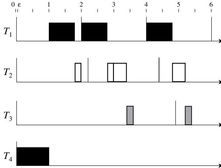
FIGURE 8-16 Example on fixed-priority scheduling and priority-ceiling protocol. ( T_1 = (\epsilon, 2, 0.8; [Black; 0.8]) , T_2 = (\epsilon, 2.2, 0.4) , T_3 = (\epsilon, 5, 0.2; [Shaded; 0.2]) , T_4 = (10, 1; [Black; 1.0]) ).
