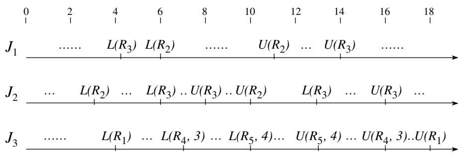
FIGURE 8–1 Examples of critical sections
