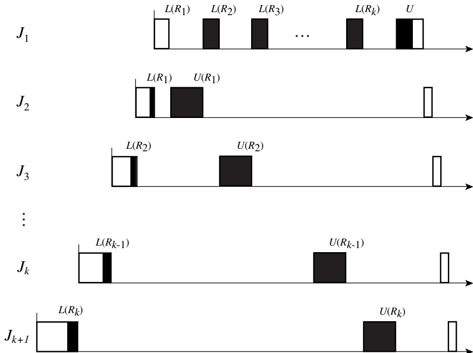
FIGURE 8–9 A worst-case blocking scenario for priority-inheritance protocol.
